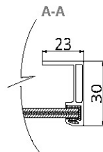
Mounting Hole
